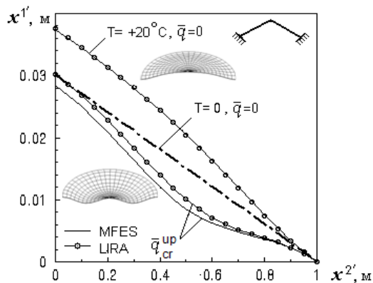
Figure 5 – Preheating shape of deformation and buckling shape of the conical shell
