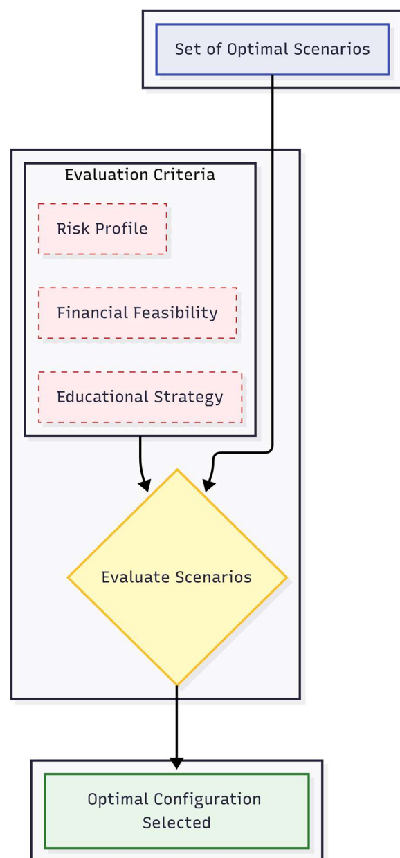
Figure 7 – Model of the Multi-Objective Fitness Evaluation Function
