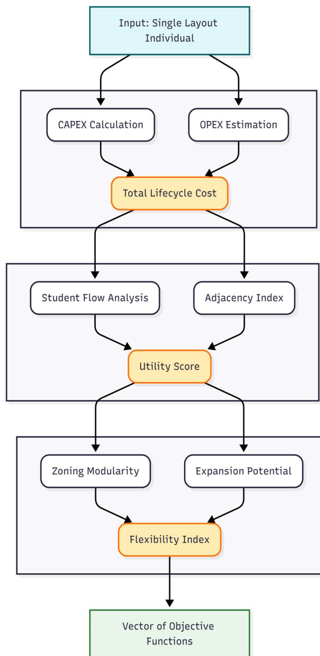
Figure 2 – Conceptual Model of the Method's Implementation
