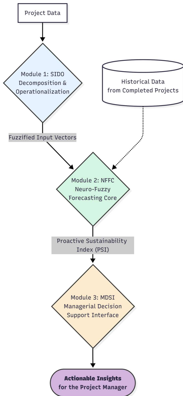
Figure 1 – Conceptual Architecture of the Proposed Method
